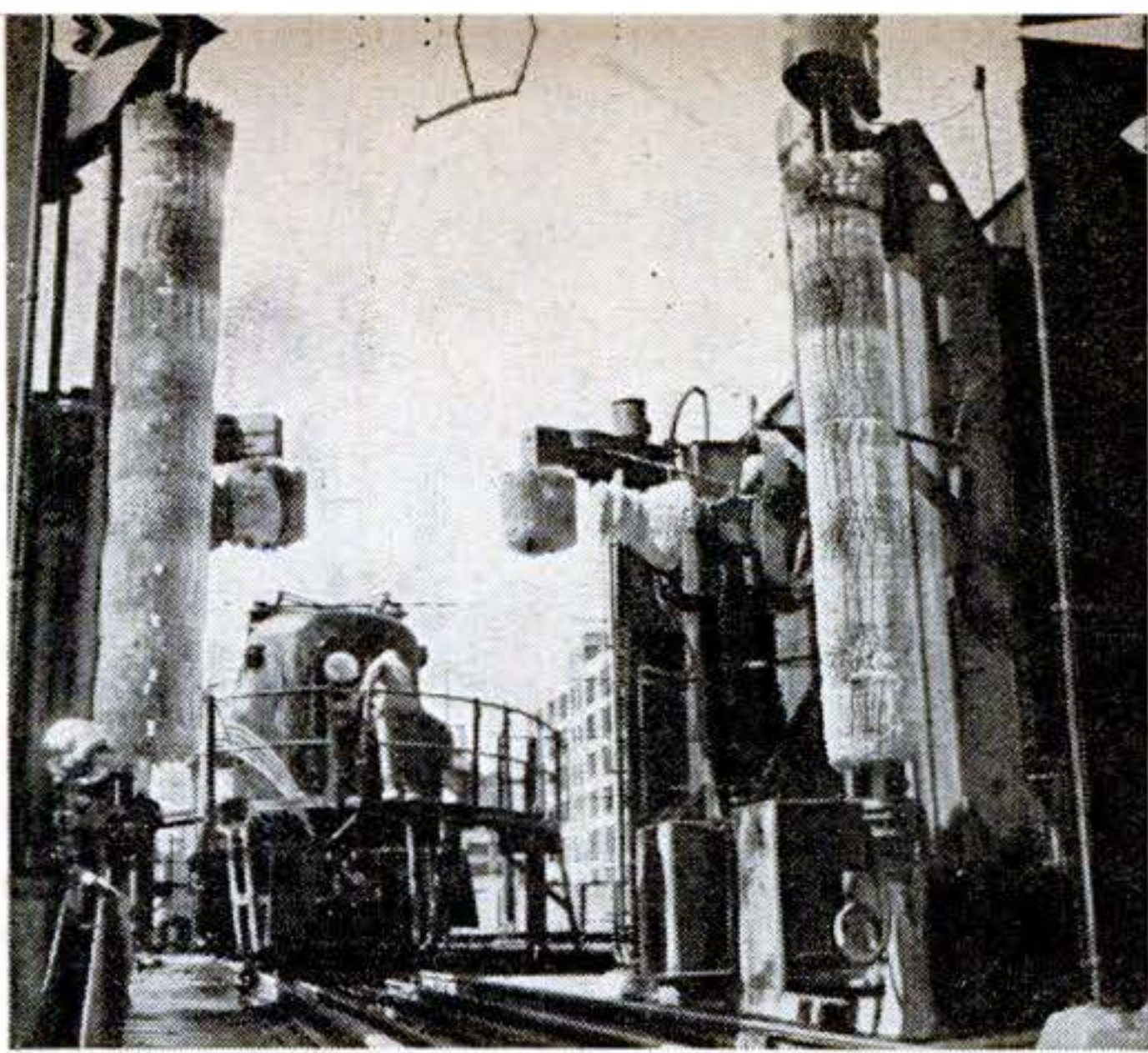
3. Front end gets the same treatment while the first set of rotary brushes, three on a side, wait in foreground to begin the real scrubbing. Engine reaches this point under its own power.
